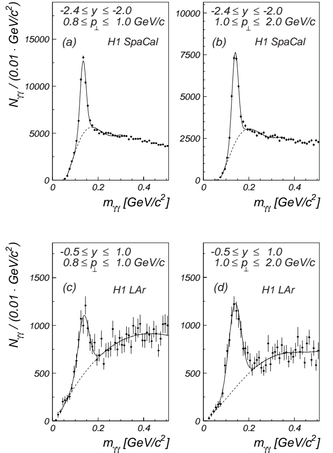
Fig. 1a–d. Two-photon invariant mass distributions reconstructed in the SpaCal calorimeter a, b and in the Liquid Argon calorimeter c, d . The full curves show fits of a sum of a Gaussian and a background distribution (dashed curves) as described in the text
