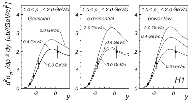
Fig. 5. The \pi^0 cross section as a function of rapidity y for the transverse momentum range 1.0 \leq p_{\perp} \leq 2.0 GeV/c. The curves are the predictions of PYTHIA, labelled with the corresponding k_{\perp 0} values, as described in the text. No additional cutoff on k_{\perp} is applied (see text)
