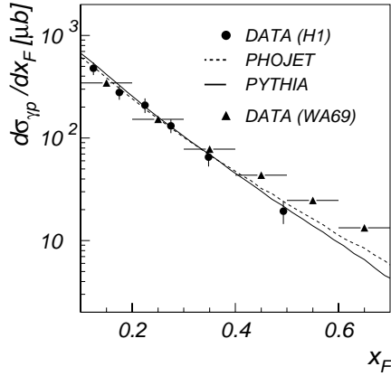
Fig. 6. Inclusive \pi^0 photoproduction cross section as a function of Feynman x . The curves are the predictions of the PHOJET (dashed) and PYTHIA (full) models. The H1 data, at \sqrt{s_{\gamma p}} \approx 208 GeV, as well as the MC model predictions, are obtained in the rapidity range -3.5 \leq y \leq -1.5 . The data of the Omega Photon Collaboration (WA69), at \sqrt{s_{\gamma p}} \approx 12.3 GeV, were derived as described in the text
