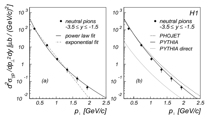
Fig. 4. a Inclusive \pi^0 photoproduction cross section as a function of transverse momentum p_\perp (circles), for the rapidity region -3.5 \leq y \leq -1.5 . The dash - dotted curve is an exponential fit to the data in the range 0.3 \leq p_\perp \leq 1.6 GeV/c; the full curve is the result of a power law fit to all data points (see text). b Same cross section as in a compared to predictions of PHOJET and PYTHIA. In addition, the contribution of direct photon interactions in PYTHIA is shown
