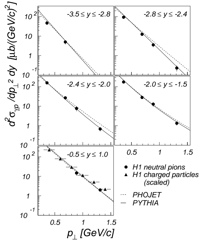
Fig. 3. Inclusive \pi^0 photoproduction cross section as a function of transverse momentum p_\perp in intervals of laboratory rapidity y (full circles). The triangles are the corresponding cross section values for charged pions in the pseudorapidity range |\eta| \leq 1.5 , derived from [1] by subtracting a fraction of 17.5% to account for the “non-pion” contribution, and then dividing by the isospin factor 2 (see text). The curves are the predictions of the PHOJET (dashed) and PYTHIA (full) event generators for neutral pions
