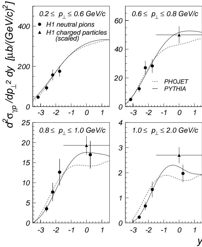
Fig. 2. Inclusive \pi^0 photoproduction cross section as a function of laboratory rapidity y in intervals of transverse momentum p_\perp (full circles). The triangles are the corresponding cross section values for charged pions, derived from [1] by subtracting a fraction of 17.5% to account for the “non-pion” contribution, and then dividing by the isospin factor 2 (see text). The curves are the predictions of the PHOJET (dashed) and PYTHIA (full) event generators for neutral pions. The \pi^0 points were bin - centre corrected; the charged pion data span the pseudorapidity interval -1.5 < \eta < 1.5
